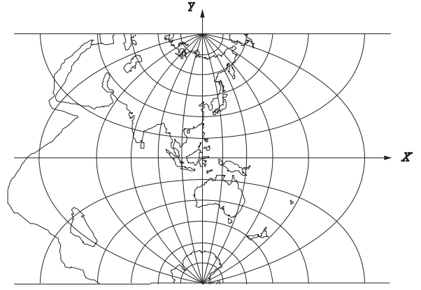
Figure 5 Transverse Mercator projection graticule interval 15^\circ , central meridian \lambda_0 = 120^\circ \text{E}
