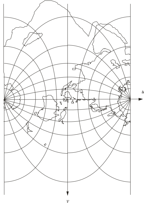
Figure 4 Transverse Mercator (TM) projection graticule interval 15°, central meridian \lambda_0 = 120^\circ \text{E}
